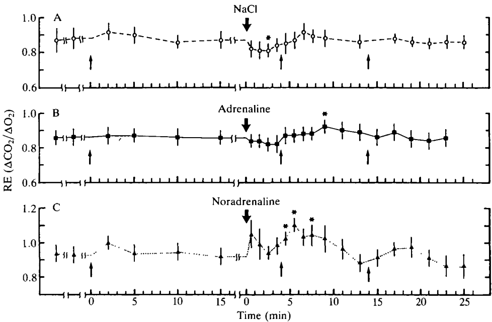
Fig. 4. The influence of saline vehicle, adrenaline and noradrenaline on the instantaneous respiratory gas exchange ratio ( \text{RE} = \Delta\text{CO}_2/\Delta\text{O}_2 ) across the gills of the rainbow trout. Other details as in legend of Fig. 1.
