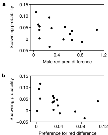
Figure 4 Relationship between the divergence among populations in male signal colour and female preference for red, and reproductive isolation between populations. Values given are for pairs of populations and are corrected for phylogeny. a , Difference in area of red coloration in males correlates negatively with spawning probability. b , Difference in
