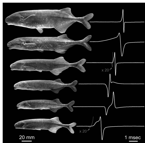
Species and morphs co-occurring in the Okano River at the abandoned village Na, near Mitzig, are shown with their electric signals. Top to bottom, Paramormyrops sp. OKA, Paramormyrops curvifrons , Paramormyrops sp. SZA, type 1 morph ( magnostipes complex), type 3 morph ( magnostipes complex), and Paramormyrops kingsleyae . Image by M. E. Arnegard and D. T. Reid.
