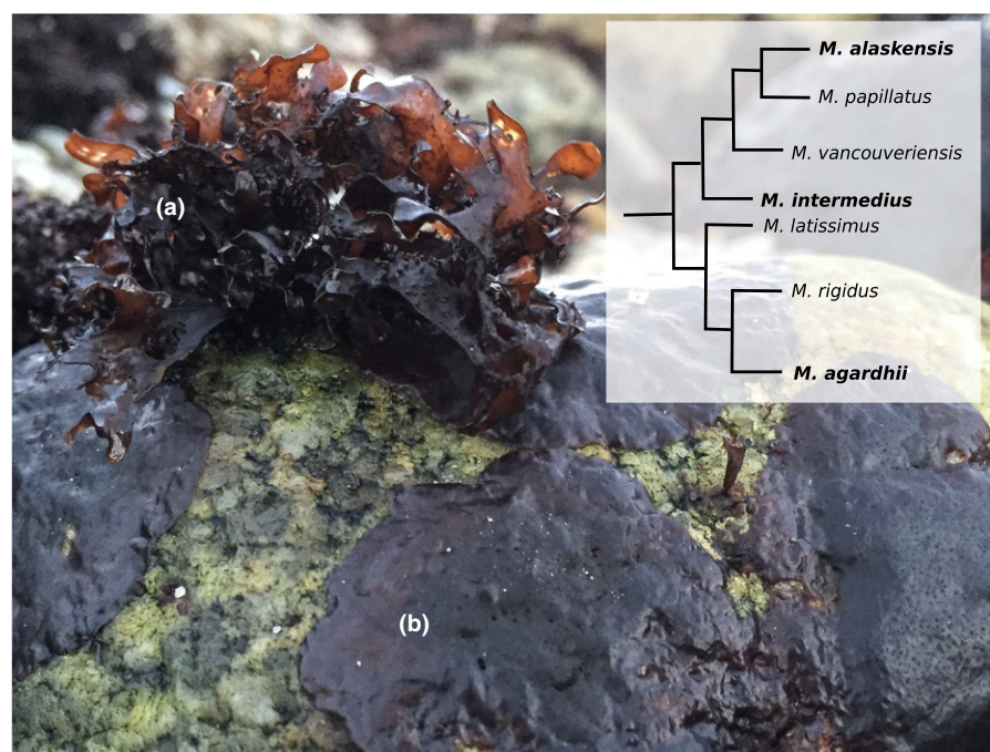
FIGURE 1 Mastocarpus exhibits alternation of heteromorphic generations: (a) The upright haploid gametophyte phase and (b) the crustose diploid sporophyte phase co-occur on rocky intertidal beaches. A phylogram of select Northeast Pacific Mastocarpus species is inset based on the three-gene consensus tree (ITS, COI and rbcL ) from Lindstrom et al. (2011); the three cryptic species present in this study are indicated in bold font. Photograph by B. Clarkston
