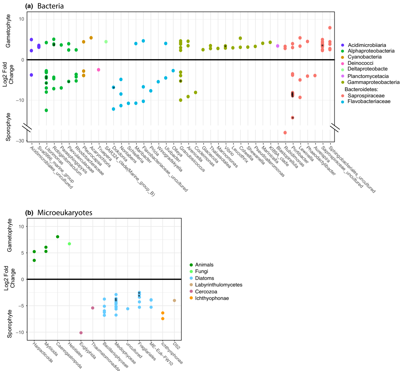
FIGURE 5 Differential abundance analysis (DESeq2) comparing sporophyte and gametophyte samples. Each circle represents an OTU with significantly different relative abundance, after FDR correction. OTUs present in either the sporophyte or gametophyte core are indicated with asterisks
