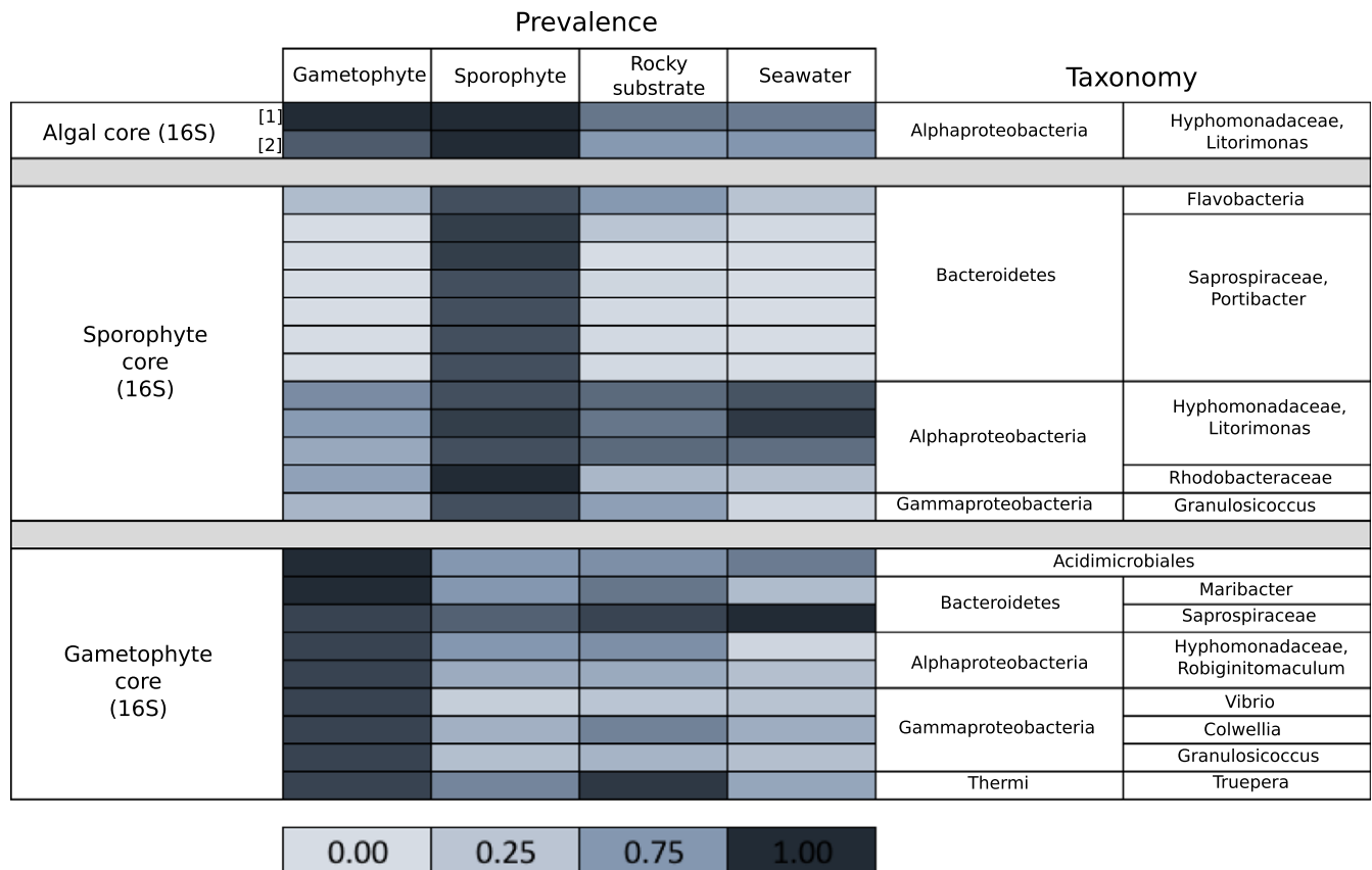
FIGURE 4 Core bacterial OTUs identified in \geq 90\% individuals from (1) all Mastocarpus samples, (2) encrusting sporophytes and (3) upright gametophytes, respectively. The groups from which core OTUs were identified are given along the y-axis, and the prevalence of each OTU is presented for gametophyte, sporophyte, rock and seawater samples (x-axis). [1] This OTU was also a member of both the sporophyte and gametophyte cores, but is only presented here. [2] This OTU was also a member of the sporophyte core, but is only presented here
