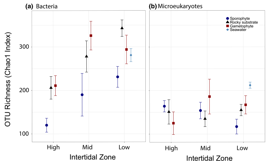
FIGURE 3 OTU richness (Chao1 index) across intertidal zones and substrate types: (a) Bacterial richness is lower on sporophytes and in the high intertidal zone; (b) the richness of microeukaryote OTUs does not significantly differ across tidal heights or substrate types, with the exception of seawater having significantly greater average richness. Data presented are mean OTU richness \pm standard error [Colour figure can be viewed at wileyonlinelibrary.com ]
