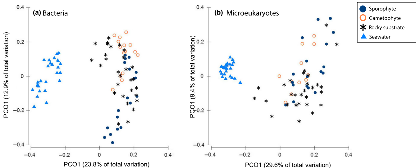
FIGURE 2 Principal coordinates analysis of unweighted UniFrac distance comparing microbial communities on each substrate type [Colour figure can be viewed at wileyonlinelibrary.com ]
