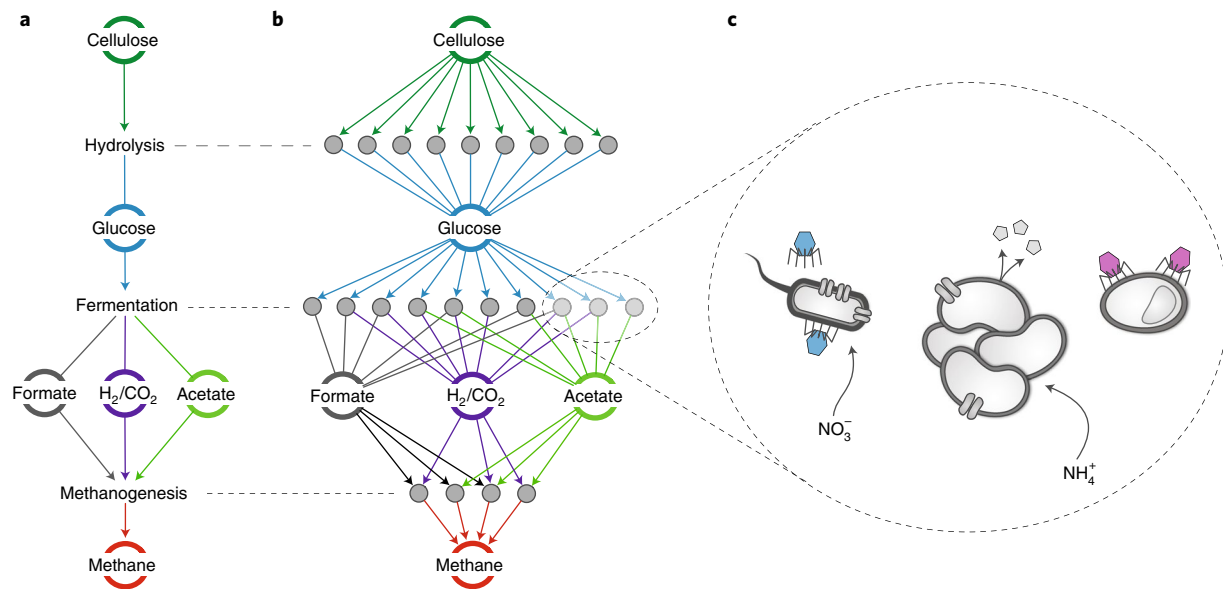
Fig. 3 | Functional redundancy in methanogenic communities (schematic illustration). a , Illustration of a typical metabolic network spanned by microbial communities in methanogenic cellulose-fed bioreactors, driving the catabolism of cellulose to methane. Circles represent substrates or end-products, and edge colour indicates the associated substrate. b , Expansion of each catabolic step, showing multiple distinct organisms capable of performing the same reaction. Filled dots represent distinct population genomes. Schematic illustration of roughly analogous findings in ref. 17 . c , Focus on three seemingly redundant organisms, catabolizing glucose to acetate. Realized niche differentiation and coexistence can be enabled by trait differences beyond the type of substrates used, potentially including susceptibility to different phages (blue versus purple), different strategies for foraging, attachment to particles and biofilm formation, different nitrogen pools used (nitrate NO 3 - versus ammonium NH 4 + ), as well as production and resistance to different antibiotics (small pentagons).
