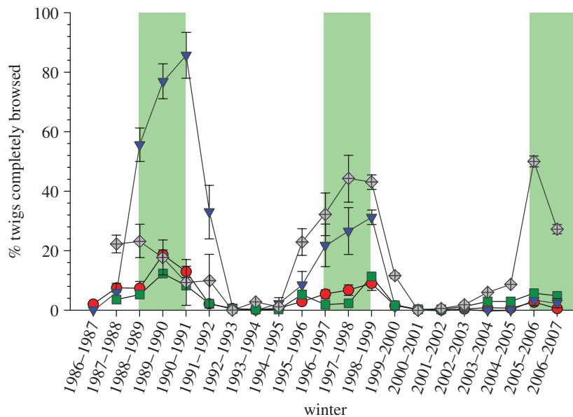
Figure 6. Percentage of willow ( Salix glauca ) and dwarf birch ( B. glandulosa ) 5 mm diameter twigs completely browsed and partly browsed in relation to the hare cycle, Klauene, Yukon. Green bars delimit the peak hare density for each cycle. An average of 600 individually tagged willow twigs and 200 birch twigs were sampled each year. Hares do not browse twigs above about 5 mm diameter, Filled circles, willow total; filled triangles, dwarf birch total; filled squares, willow partial; filled diamonds, dwarf birch partial.
