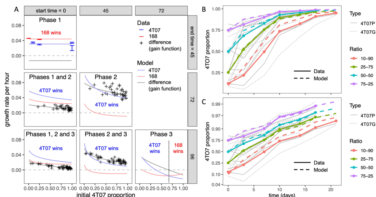
Figure 3. Mean net growth rate differences according to mathematical model and experimental data. A: Inferred mean net growth rates and mean net growth rate differences (gain functions) over different time periods, corresponding to different phases within competition assays. Columns correspond to different start times and rows to different end times of the phase(s) under consideration. For example, the centre panel labelled 'Phase 2' corresponds to the period between 45 and 72 hours. The initial 4T07 proportion (horizontal axis) is measured at the start of the respective period and the growth rate (vertical axis) is averaged over the period. Phase 1 data are from time-lapse microscopy. Other data points in the first column are from serial competition assays, such that each point corresponds to the slope of a thin grey line in B . Data points in the middle column are obtained from the competition assay data by adjusting for exponential growth during phase 1 (see Methods). Curves are the results of our mathematical model (Methods) with parameter values inferred from data (Table 1). B: 4T07 frequency dynamics across serial competition assays. Thick solid lines are averaged data (means of replicates with similar initial 4T07 proportions) and thick dashed lines are results of our mathematical model with parameter values inferred from data. Thin grey lines are data for individual experiments. A total of 10^5 cells were seeded in co-cultures and harvested and replated as indicated. 4T07 parental cells were transduced either with an empty retroviral vector (4T07P) or labelled with a GFP-encoding retrovirus (4T07G). The ratios of GFP to unlabelled cells were estimated by flow cytometry. C: Logit-transformed 4T07 frequency dynamics. This panel shows the same data as B but with a logit-transformed vertical axis so that the slope of each curve is equal to the mean net growth rate difference (the gain function, as described in Methods and Supplementary figure 7).
