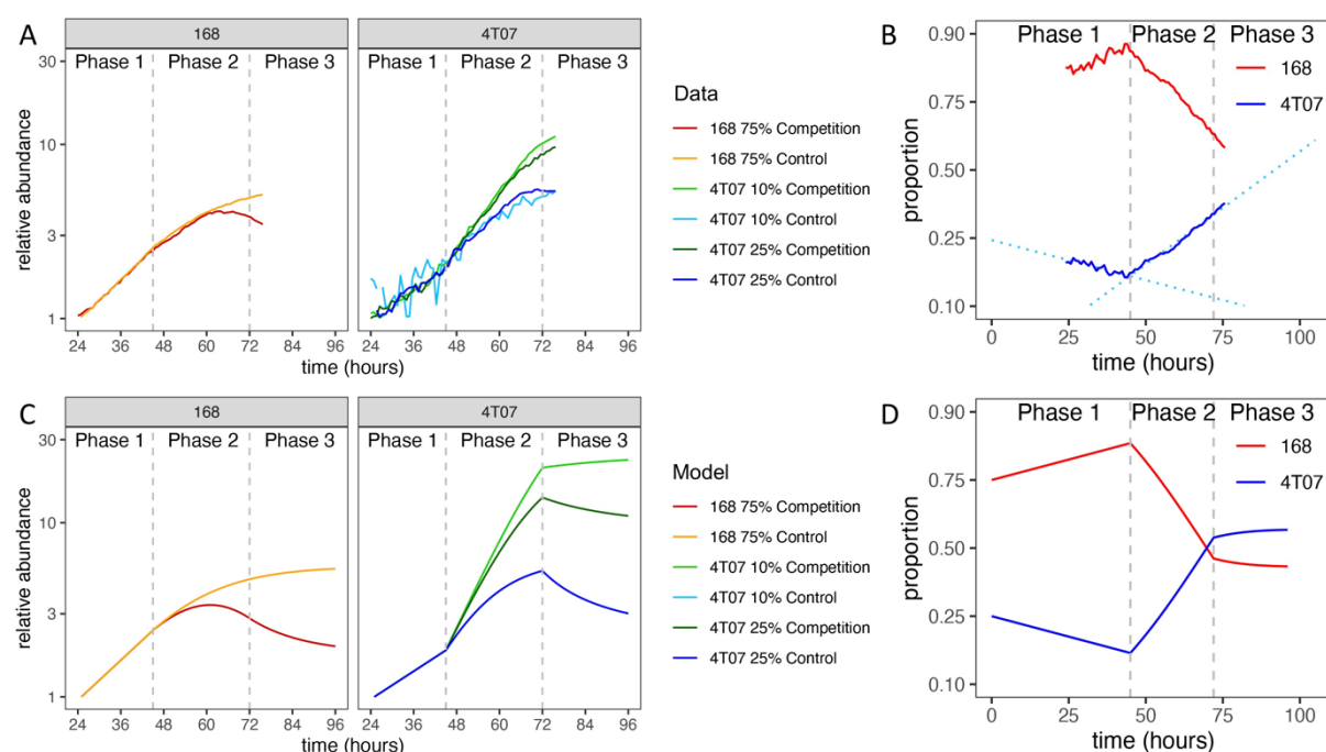
Figure 2. Normalized growth curves of homotypic and heterotypic mixes of subclones. A: The GFP fluorescence of the labeled subclone was measured by time-lapse microscopy. Cultures were seeded with 10^5 cells per well. Log-transformed data were normalized by fitting regression lines and dividing by the inferred value at 24 hours. Vertical dashed lines mark the start of phase 2 (45 hours) and phase 3 (72 hours). B: Frequency dynamics. Curves obtained by combining the results of two competition experiments: one with labelled 4T07 and the other with labelled 168. The initial 4T07 proportion was 25% in both cases. The vertical axis is logit-transformed so that the slope of each curve is equal to the difference in net growth rates at the corresponding time (see Methods). Dotted regression lines are shown to draw attention to the change of slope. C: Normalized growth curves according to mathematical model with parameter values inferred from data. The model is described in Methods and parameter values are given in Table 1. D: Frequency dynamics according to mathematical model with parameter values inferred from data.
