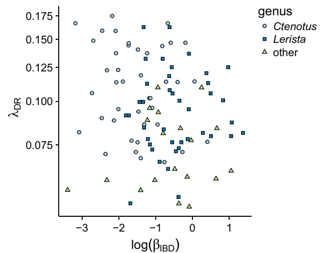
Figure 7: Relationship between population structure ( \beta_{\text{IBD}} ) and speciation rate at the tips as measured by the equal-splits ( \lambda_{\text{DR}} ). Points are coded by genera; “other” includes all non- Ctenotus /non- Lerista operational taxonomic units (fig. 2). Speciation rate and \beta_{\text{IBD}} are not correlated (phylogenetic generalized least squares; P = .47 , r = 0.004 ), suggesting that the tempo of speciation is unrelated to the extent of population structure in this clade. DR = diversification rate; IBD = isolation by distance.
