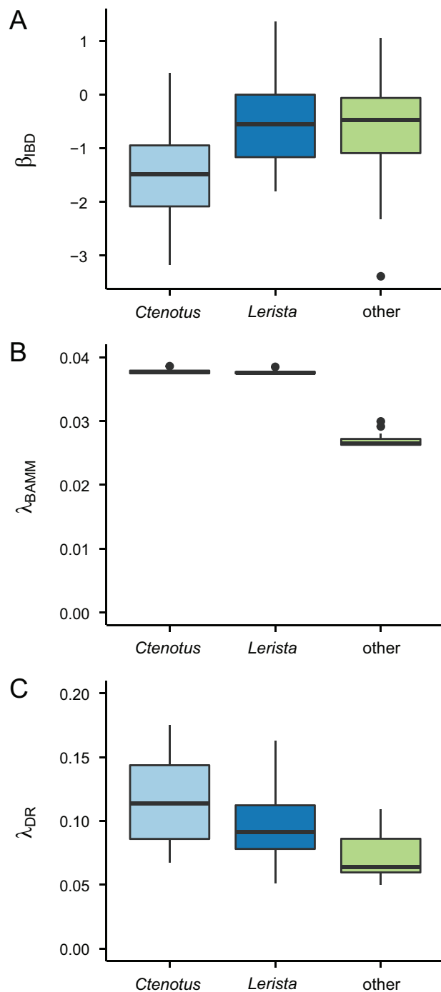
Figure 6: Distributions of population structure ( \beta_{\text{IBD}} ; A) and speciation rates (B, C) for Ctenotus , Lerista , and all other operational taxonomic units. Although Ctenotus and Lerista exhibit higher speciation rates than other sphenomorphine skinks, we see no corresponding increase in the extent of population structure. BAMM = Bayesian analysis of macroevolutionary mixtures; DR = diversification rate; IBD = isolation by distance.
