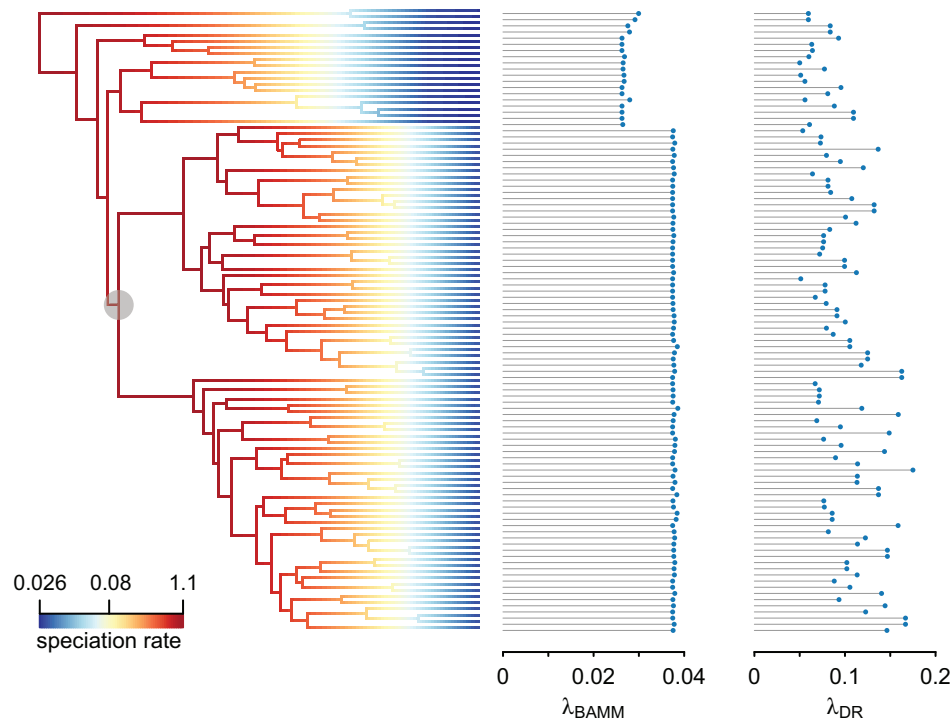
Figure 5: Variation in speciation rates across the sphenomorphine clade as estimated by two metrics for speciation rates at the tip: Bayesian analysis of macroevolutionary mixtures (BAMM) tip rates ( \lambda_{\text{BAMM}} ) and the equal-splits metric ( \lambda_{\text{DR}} ). The phylogeny depicts the BAMM-inferred speciation rates through time mapped onto a pruned phylogeny of the 104 taxa included in this study. The gray circle marks the location of the inferred rate shift in speciation rates at the base of the Ctenotus and Lerista clades. Across both metrics, speciation rate varies across the tree. DR = diversification rate.
