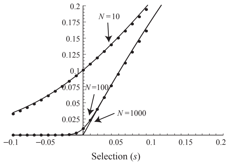
Fixation probability
