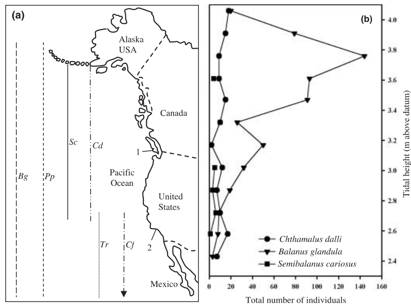
Figure 1 (a) Geographical distribution of the intertidal barnacles Balanus glandula (Bg), Pollicipes polymerus (Pp), Semibalanus cariosus (Sc), Chthamalus dalli (Cd), Tetraclita s. rubescens (Tr), and C. fissus (Cf). Arrow indicates distribution extends beyond map. Numbers represent the two collection sites: (1) Bamfield, Vancouver Island, British Columbia, Canada (48°50'N, 125°22'W), and (2) County Line, California, USA (34°06'N, 118°38'W). Distributions taken from Morris et al. (1980). (b) Vertical distribution (tidal height) of sympatric acorn barnacles B. glandula , S. cariosus and C. dalli at Bamfield (collection site 1). Total number of individuals = the number of all individuals (counted at 10-cm intervals) adjacent to vertical transects through the intertidal zone, summed over three transects.
